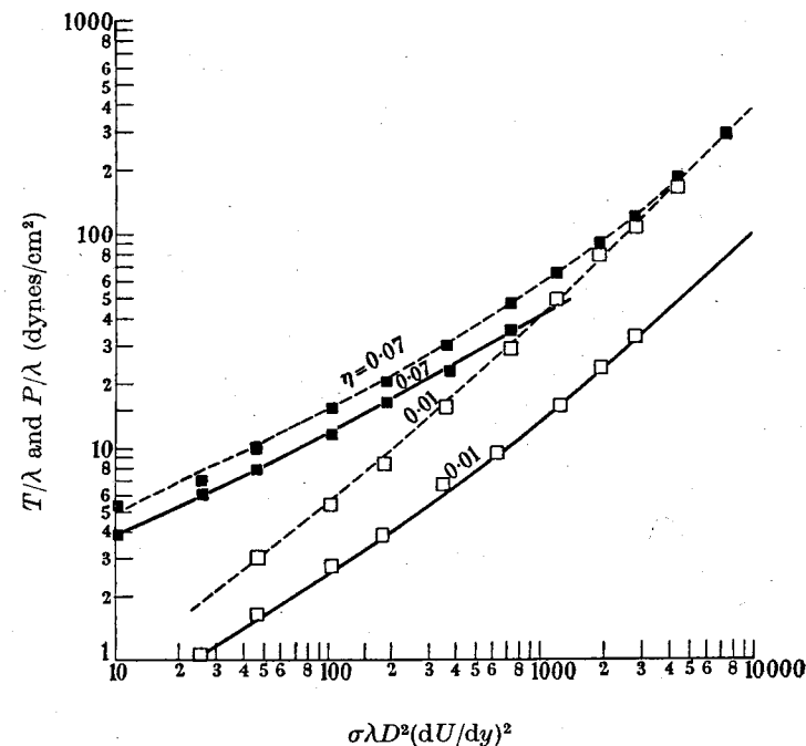
FIGURE 6. Change of fluid viscosity. The complete lines indicate grain shear stress and the broken lines grain pressure. \lambda = 11 .
