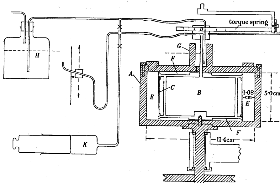
FIGURE 2. The apparatus (rotating parts shown hatched).
